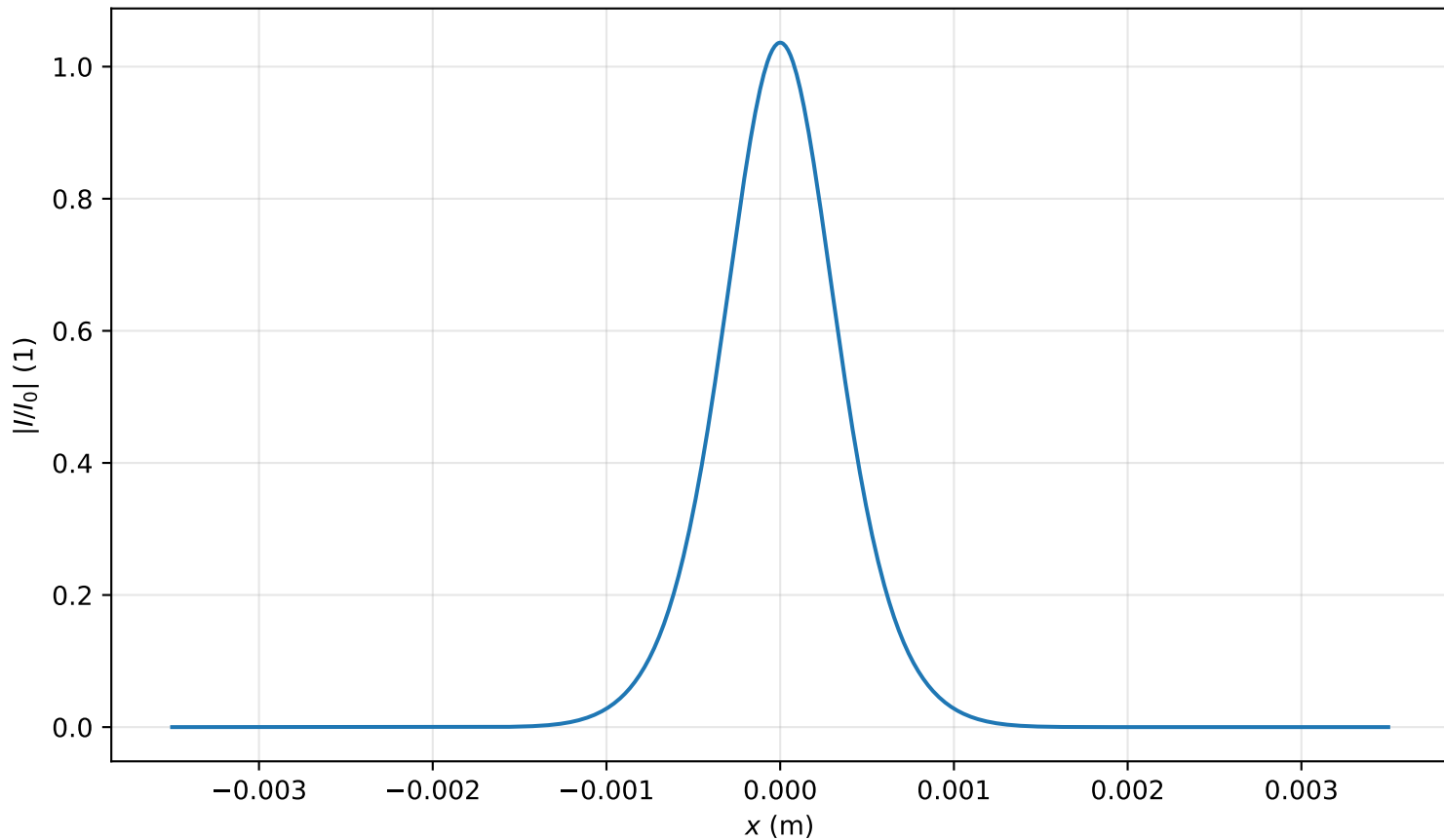
Intensity profile I(x, y = 0, z = 1.115m)/I_0 , P_{in}=0.5P_{cr} , artificial time
